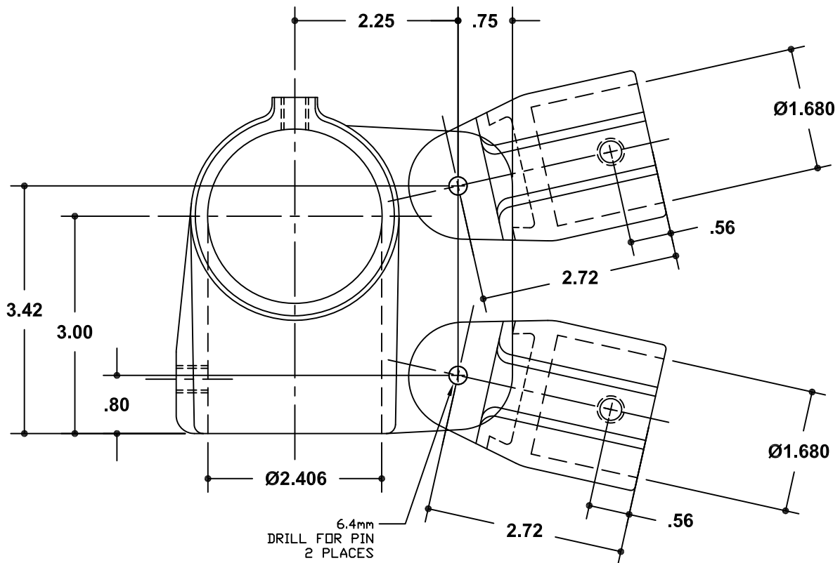
#25R-977 Tee Adjustable Brace Assembly
